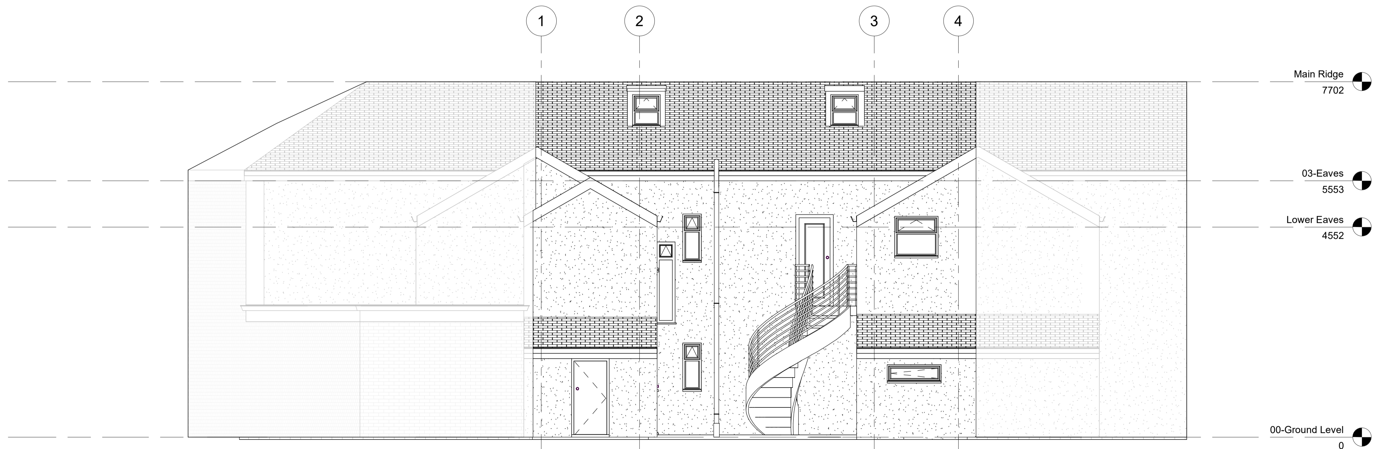
2 Elevation Rear 1 : 50
