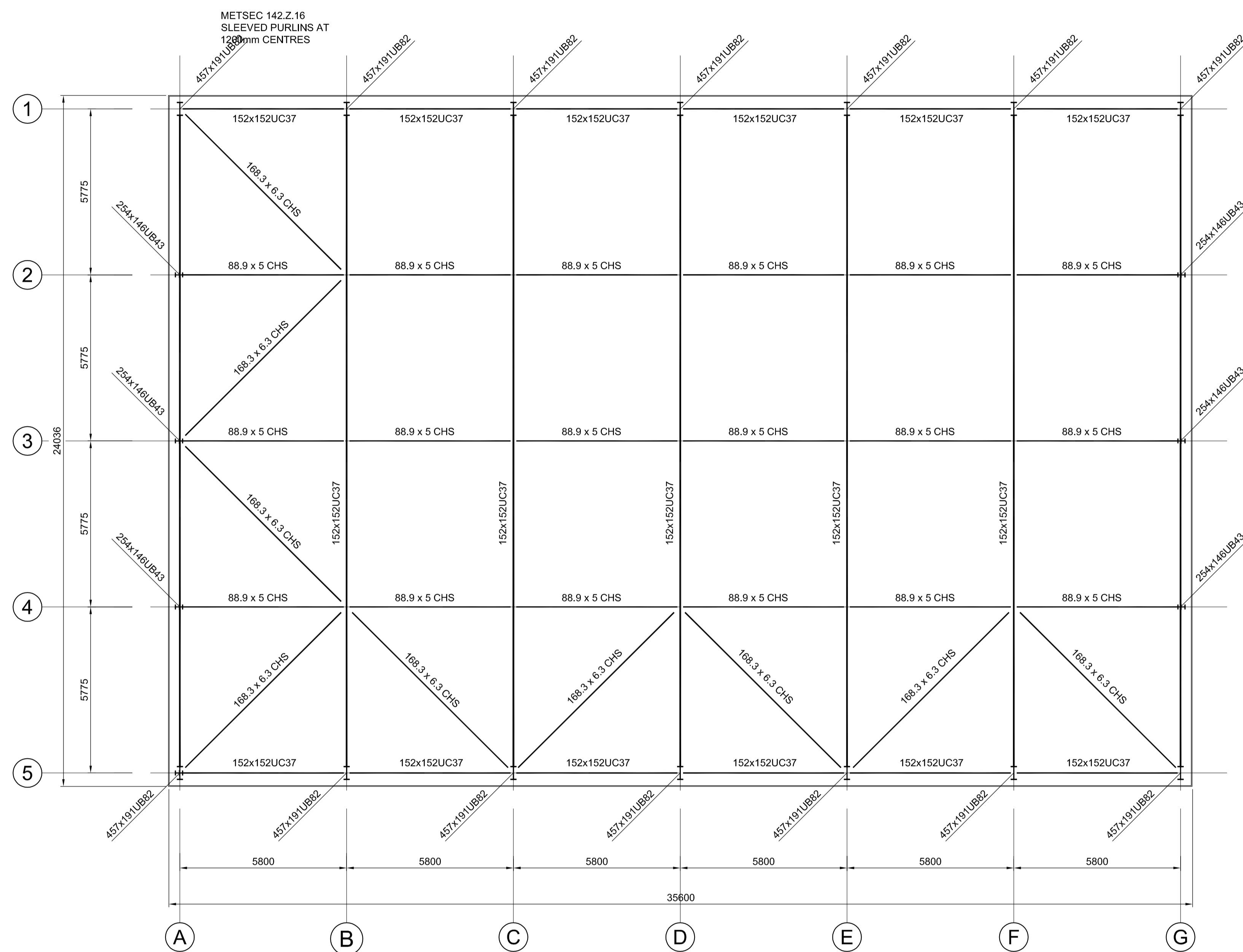
PLAN AT TRUSS BOTTOM CHORD LEVEL
