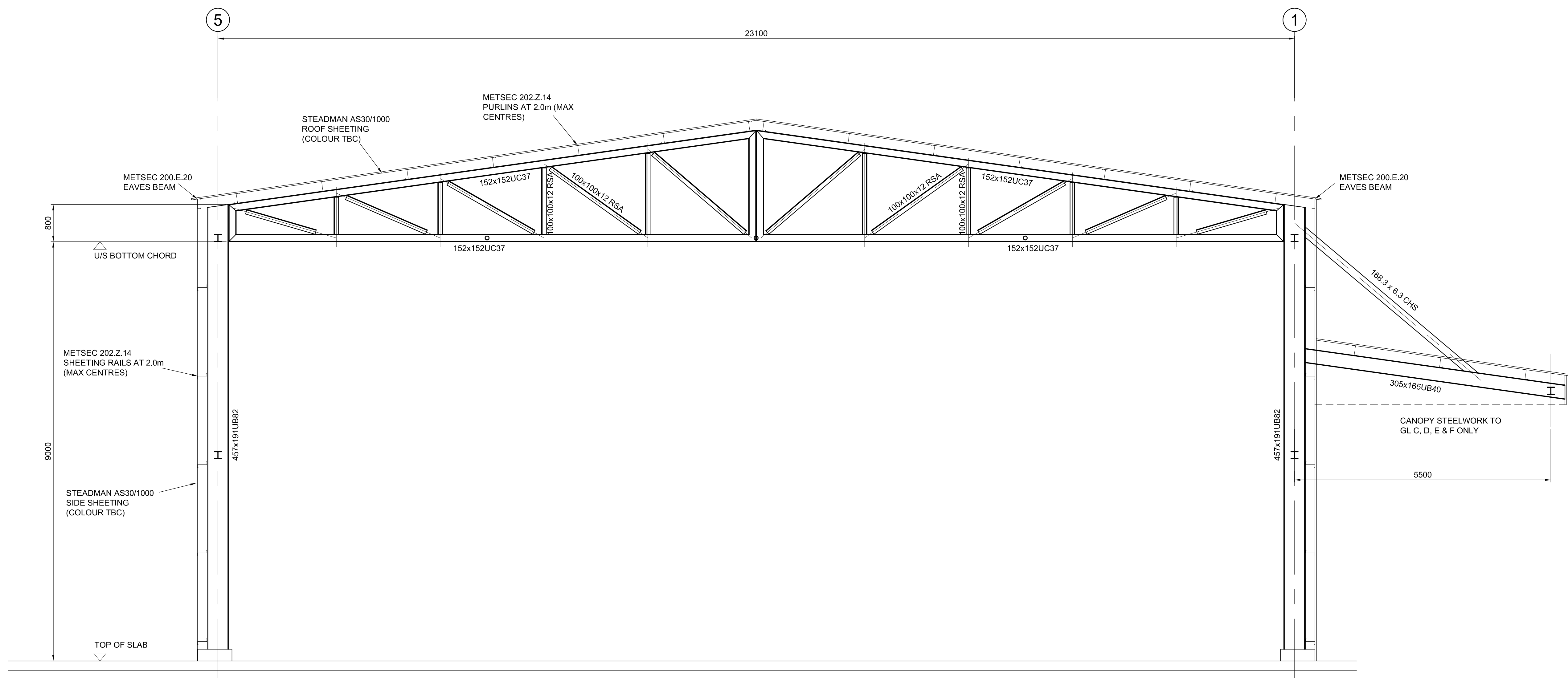
ELEVATION ON GL A - GL G
