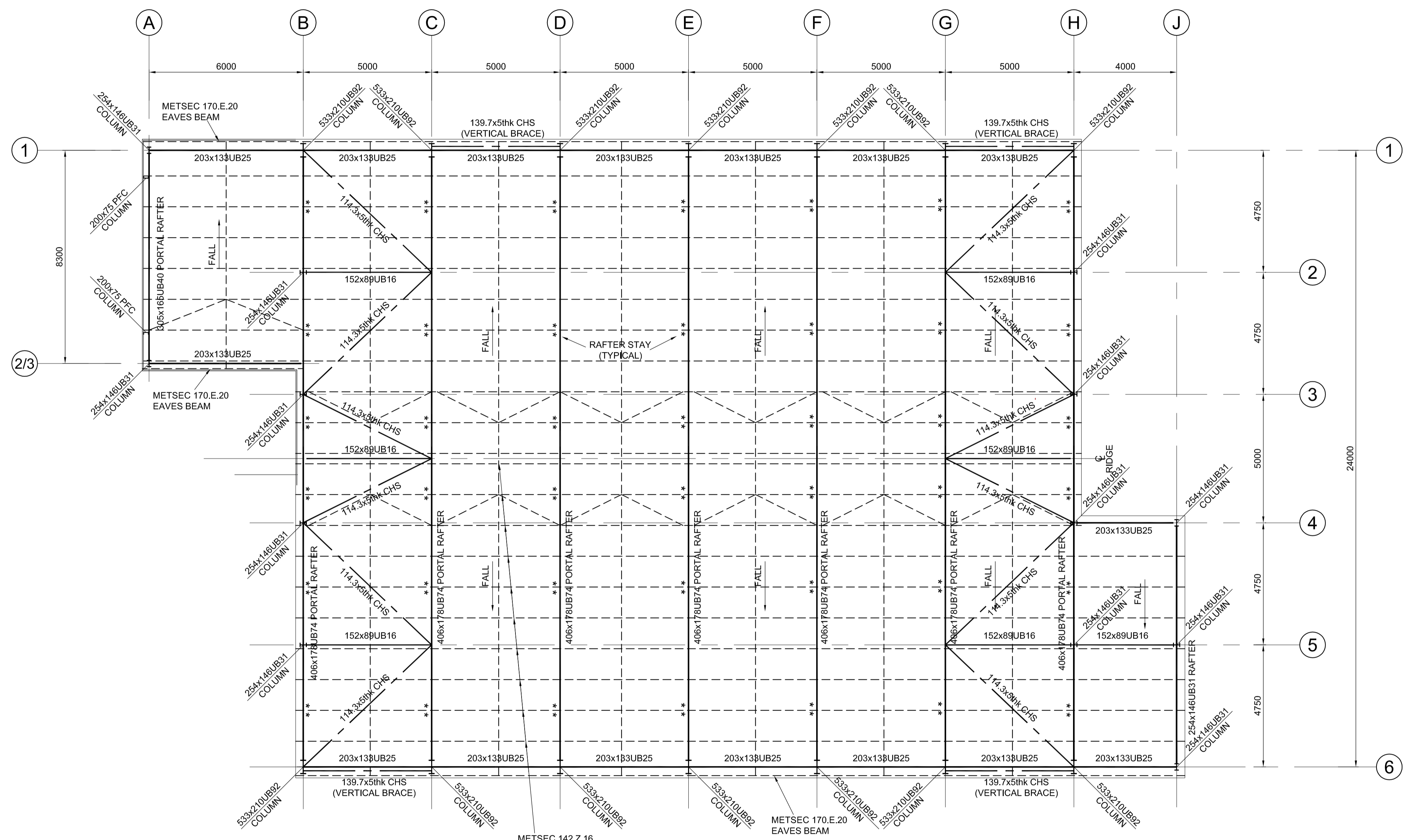
ROOF PLAN
