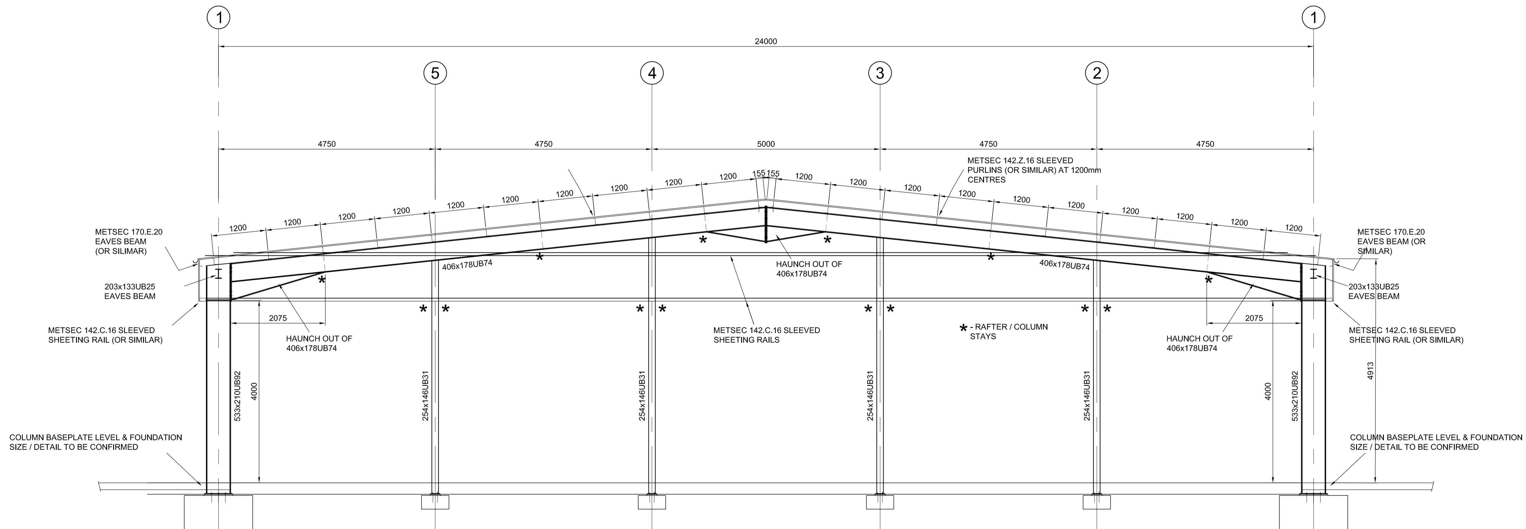
ELEVATION ON GL B
