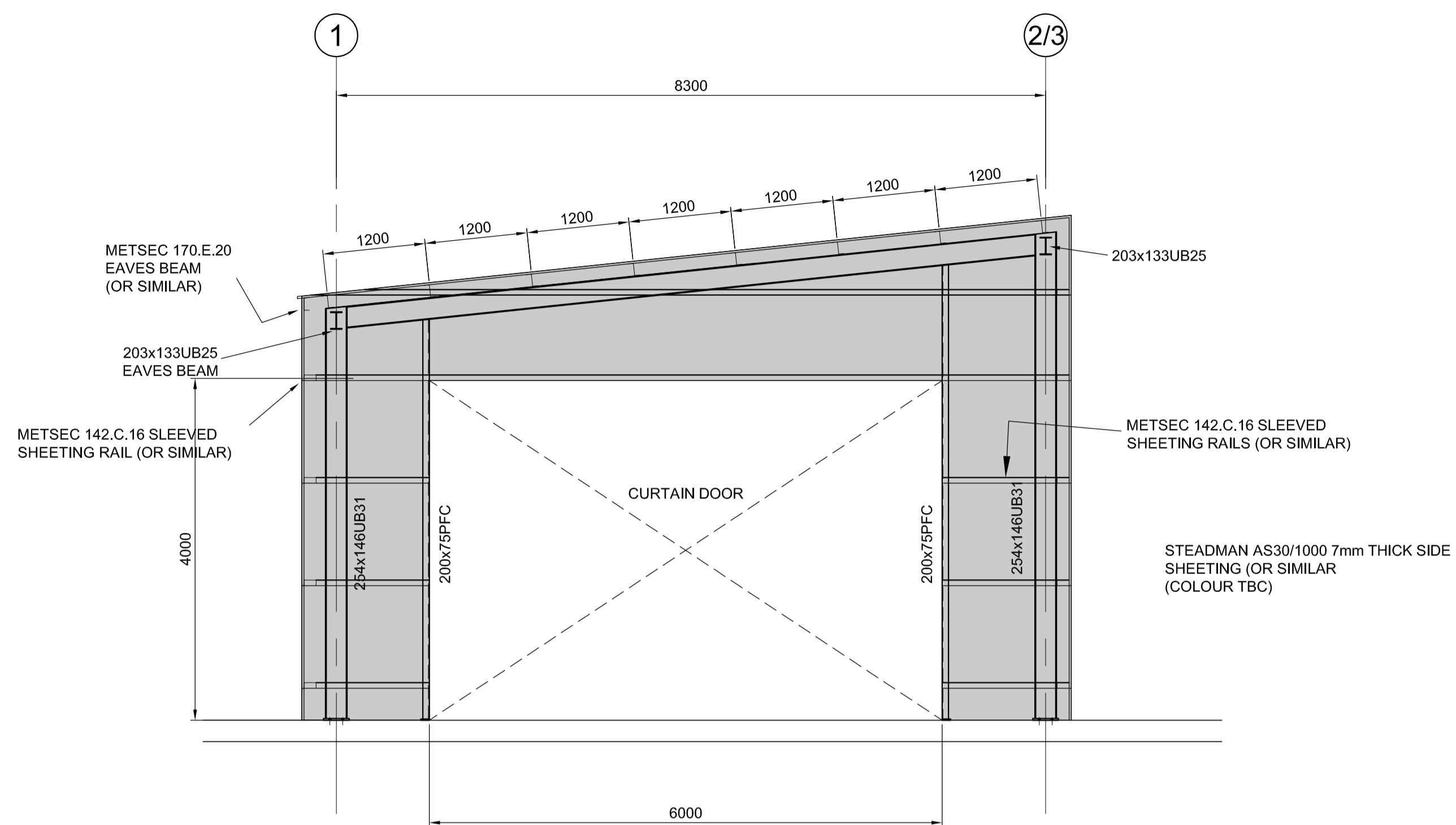
ELEVATION ON GL A
