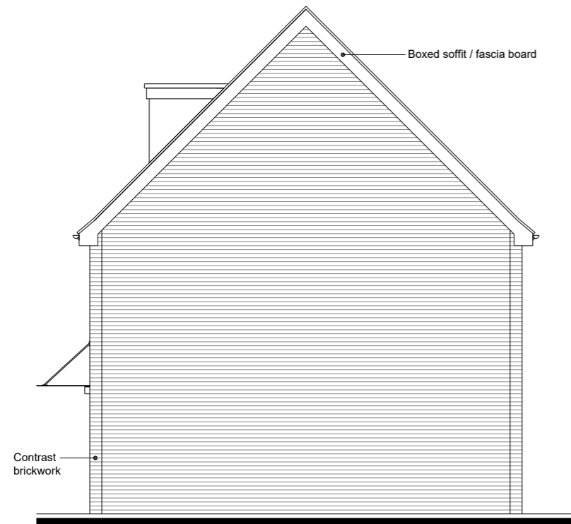
Side Elevation (AP) Left
