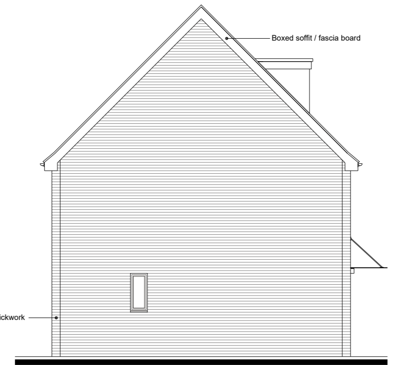
Side Elevation (AP) Right
