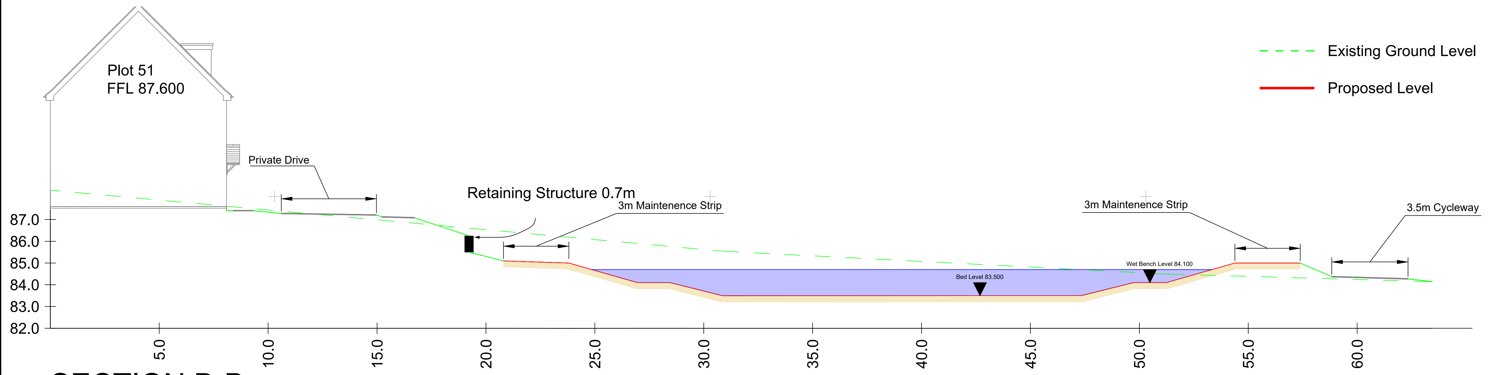
SECTION B-B
