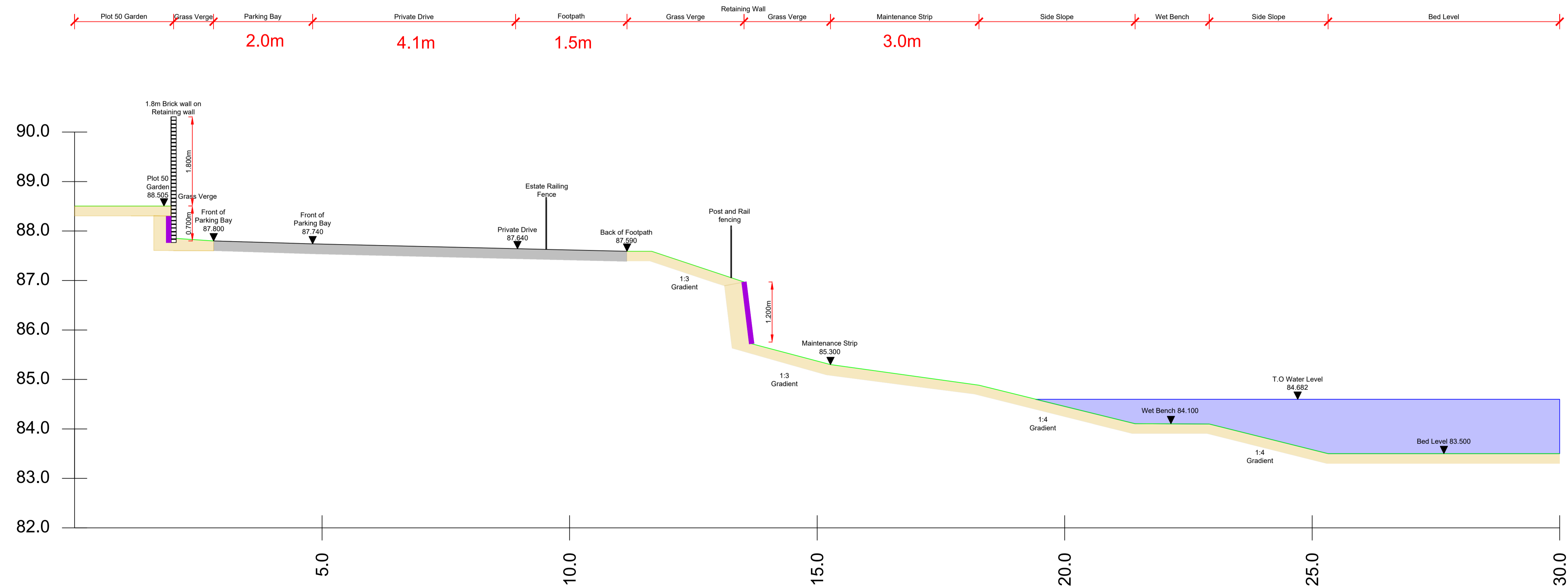
SECTION B-B
