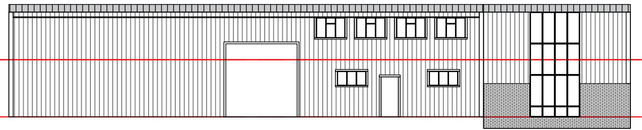
EXISTING SOUTH WEST FACADE
