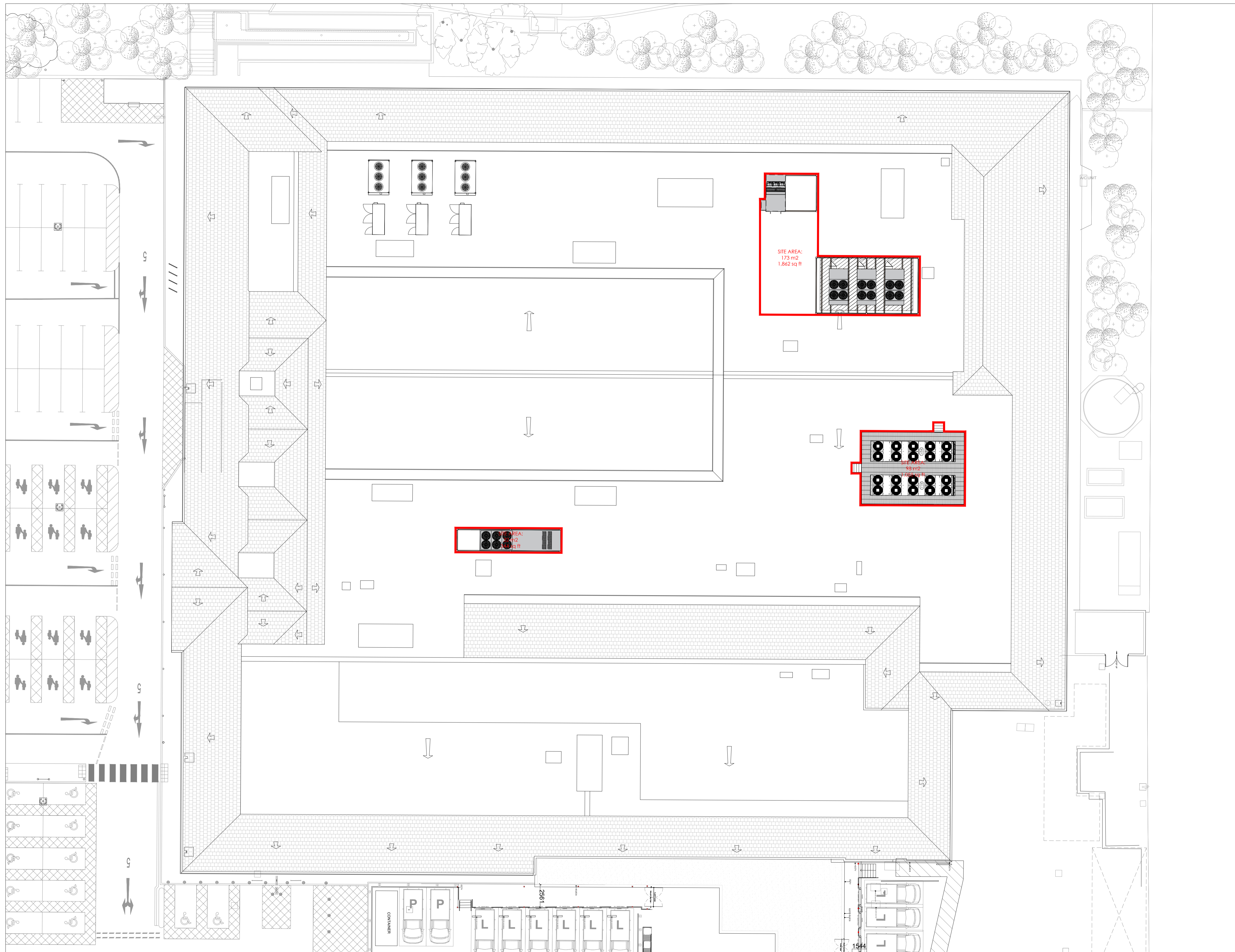
PROPOSED ROOF PLAN SCALE (1:200 @ A1)
