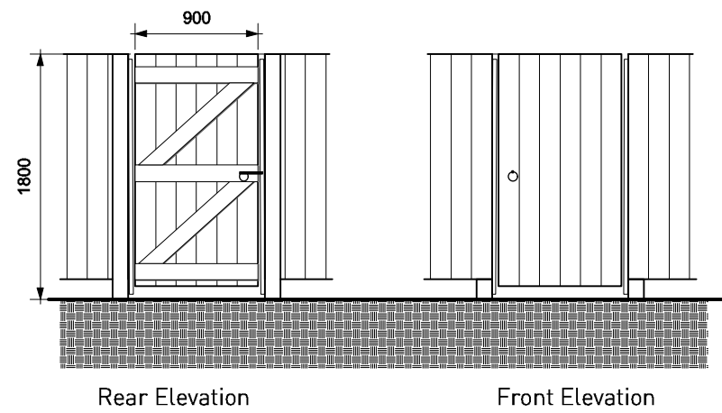
1.8M HIGH TIMBER GARDEN ACCESS GATE
