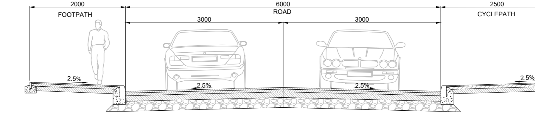
TYPICAL CROSS SECTIONS
