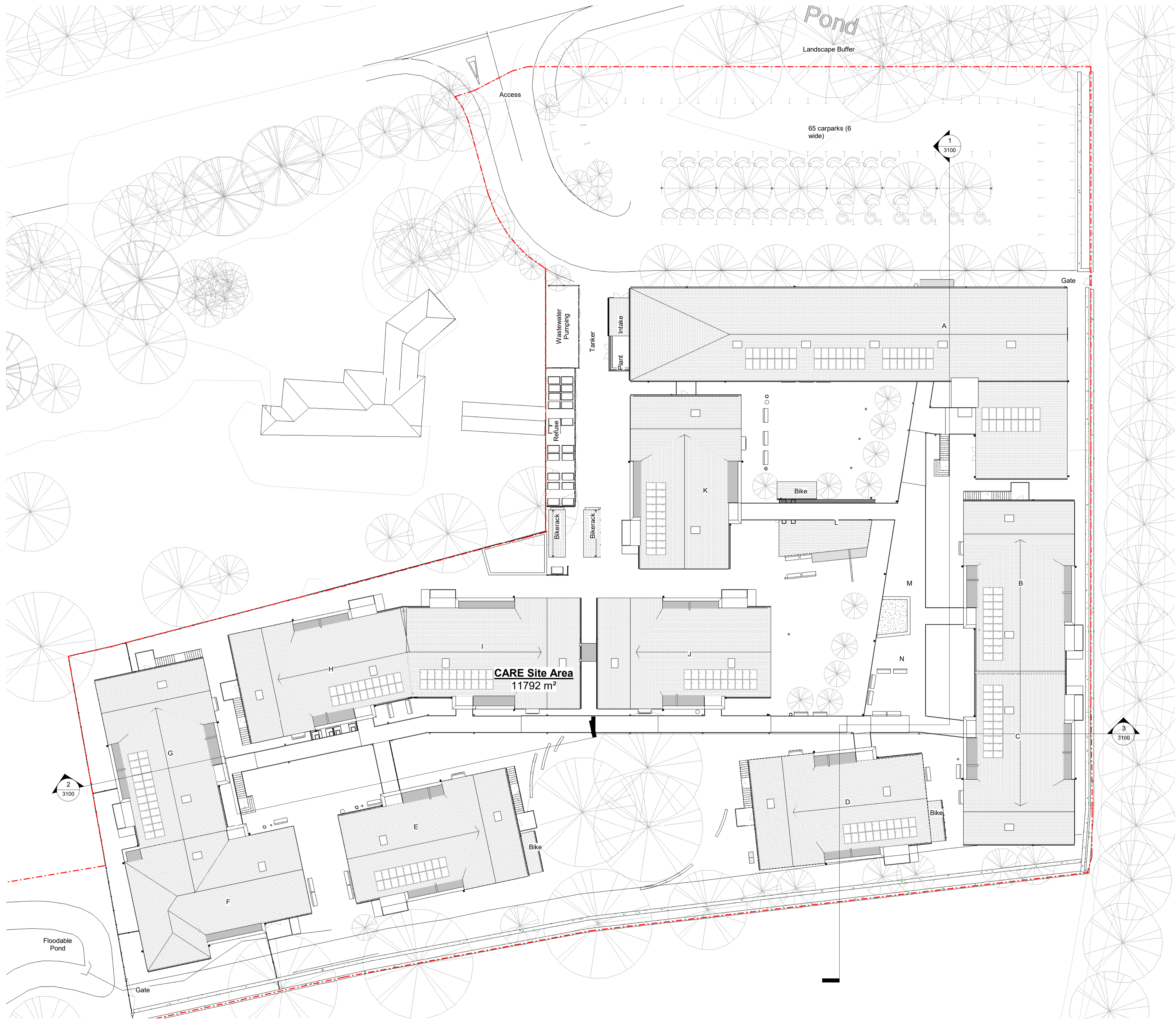
Roof Site Plan
