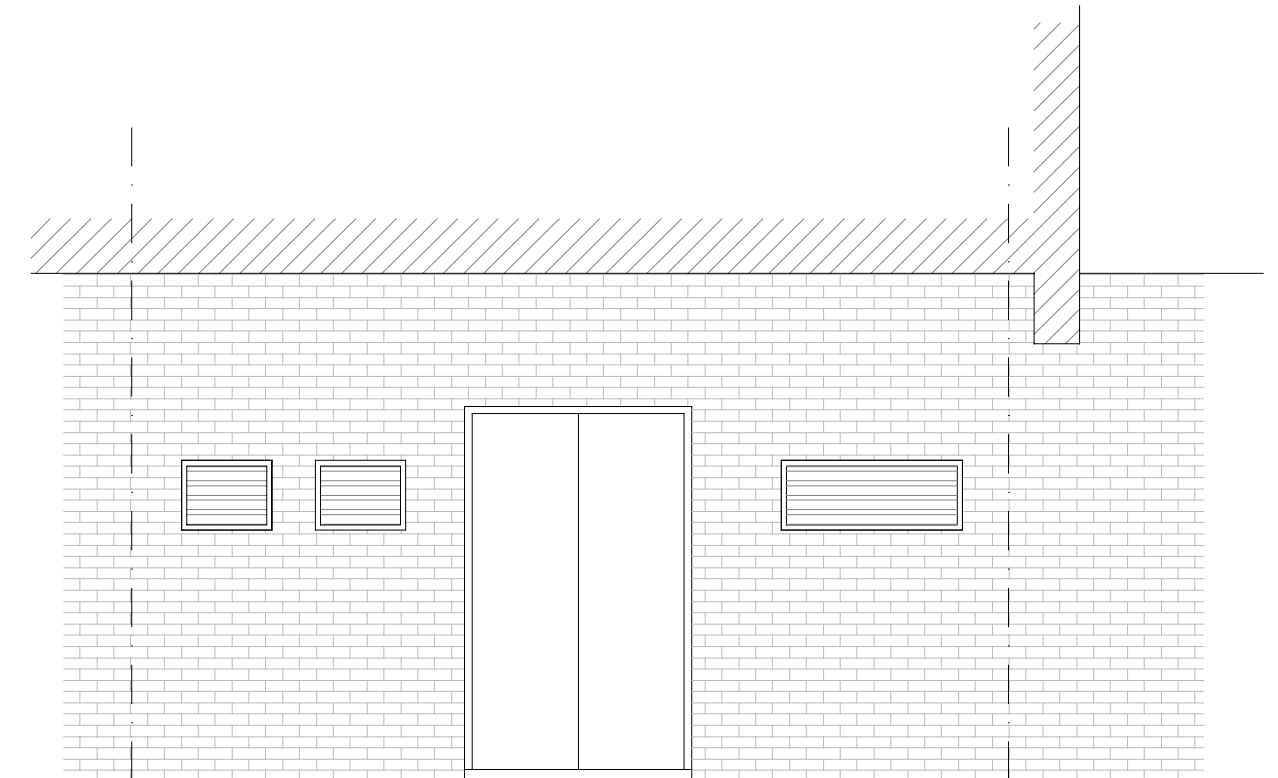
EXISTING REAR ELEVATION SOUTH WEST
