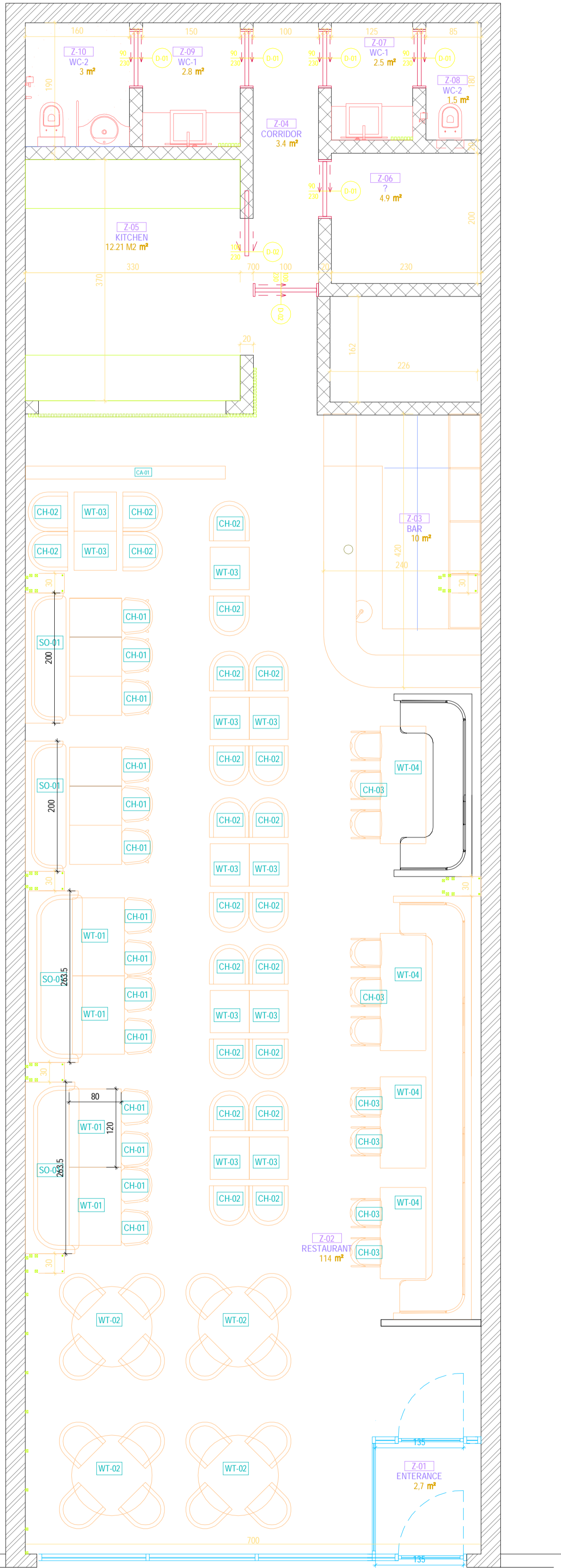
GROUND FLOOR PROPOSED PLAN SCALE 1:50
