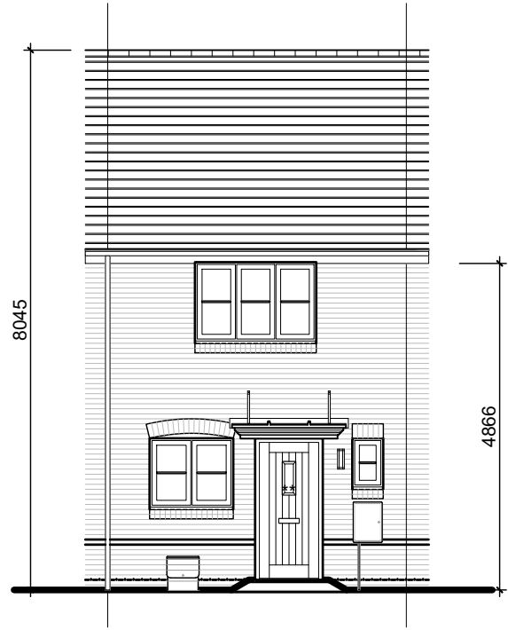
FRONT ELEVATION 1:100@A3
