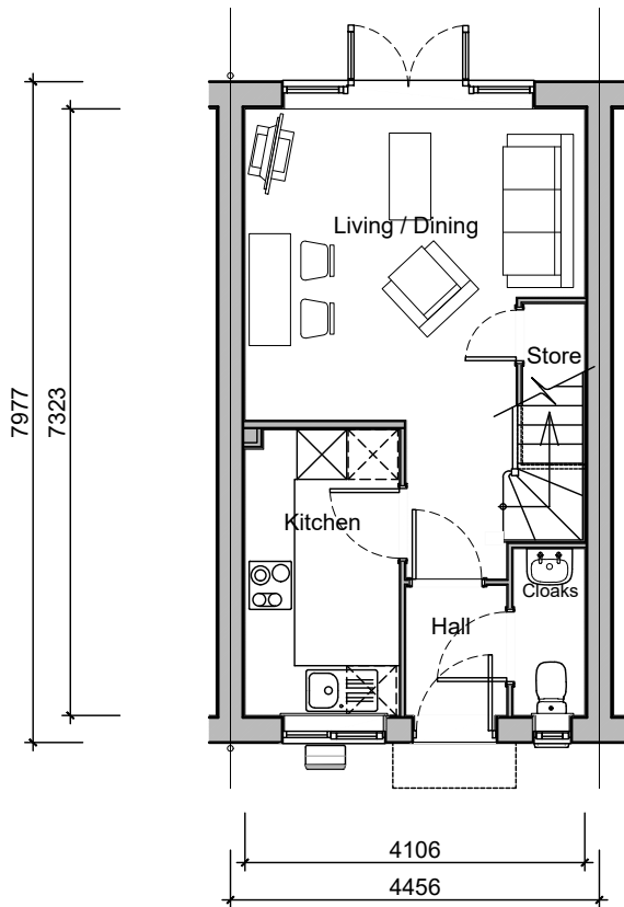
GROUND FLOOR PLAN 1:100@A3
