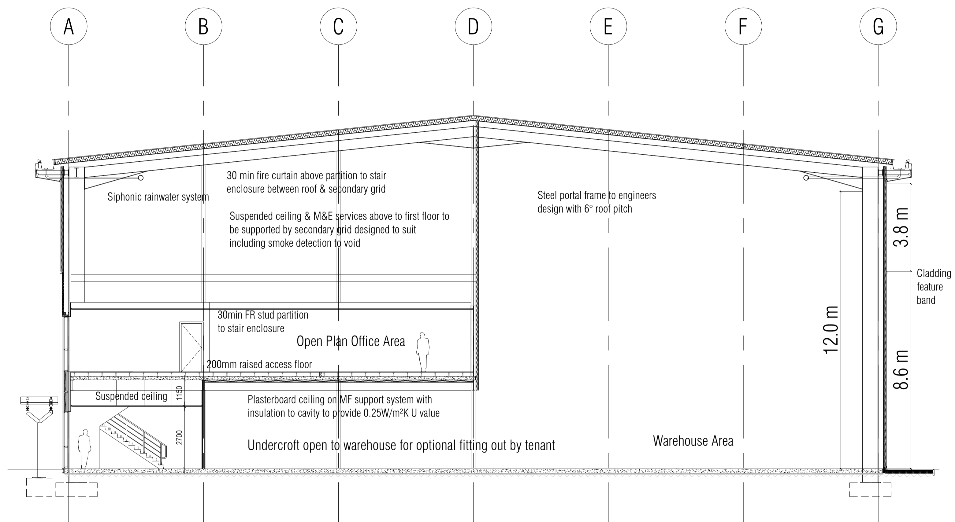
Typical Section
