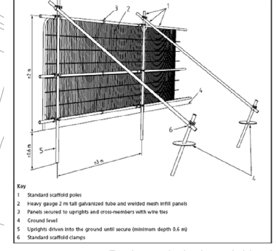
Figure 2 Default specification for protective barrier
