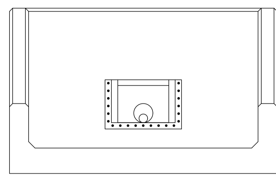
(HW3) R18B 01 1150 HEADWALL (ATHLON) WITH ATTACHED ORIFICE PLATE
