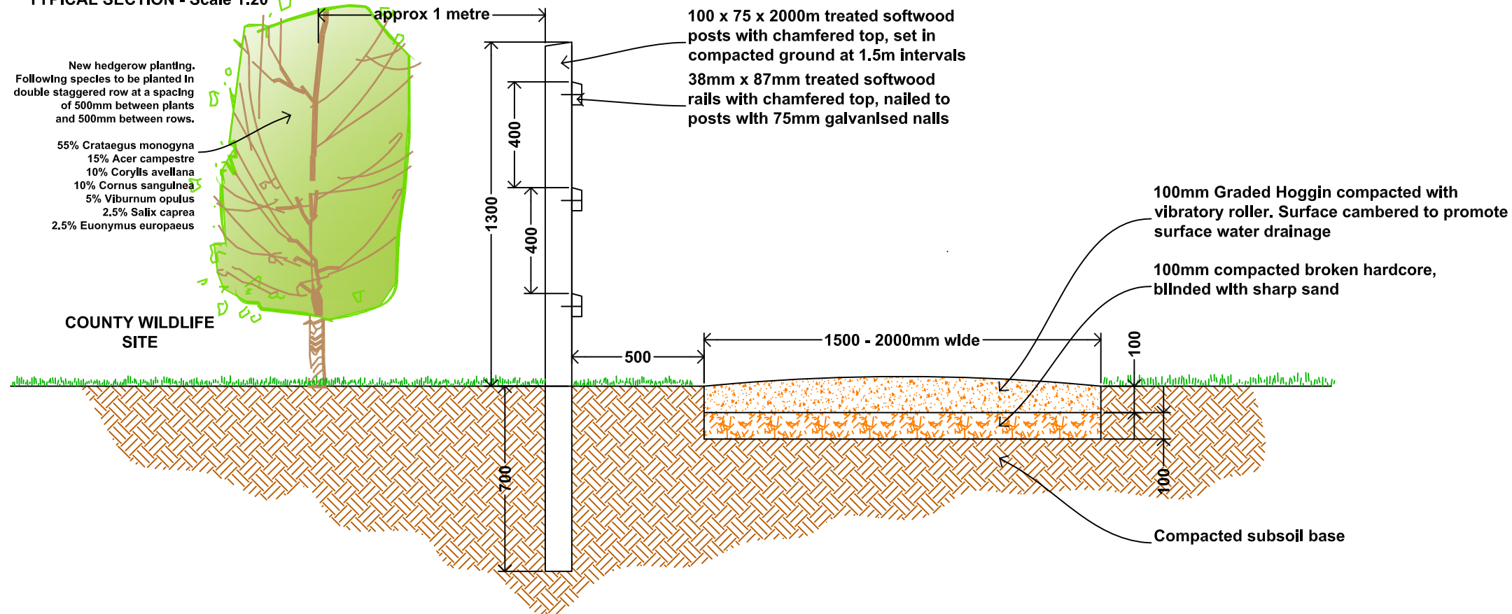
TYPICAL SECTION - Scale 1:20
