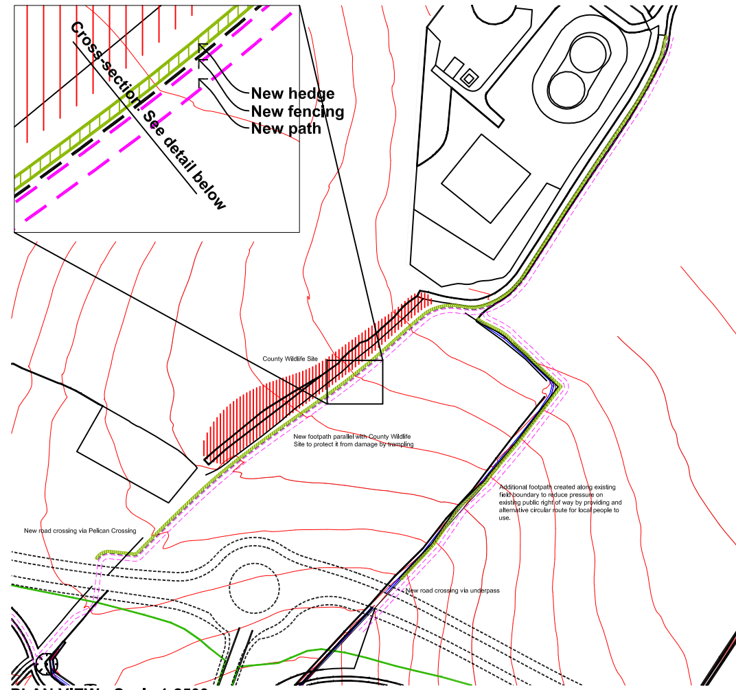
PLAN VIEW - Scale 1:2500
