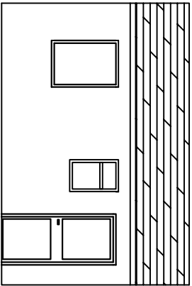
PROPOSED FRONT ELEVATION
