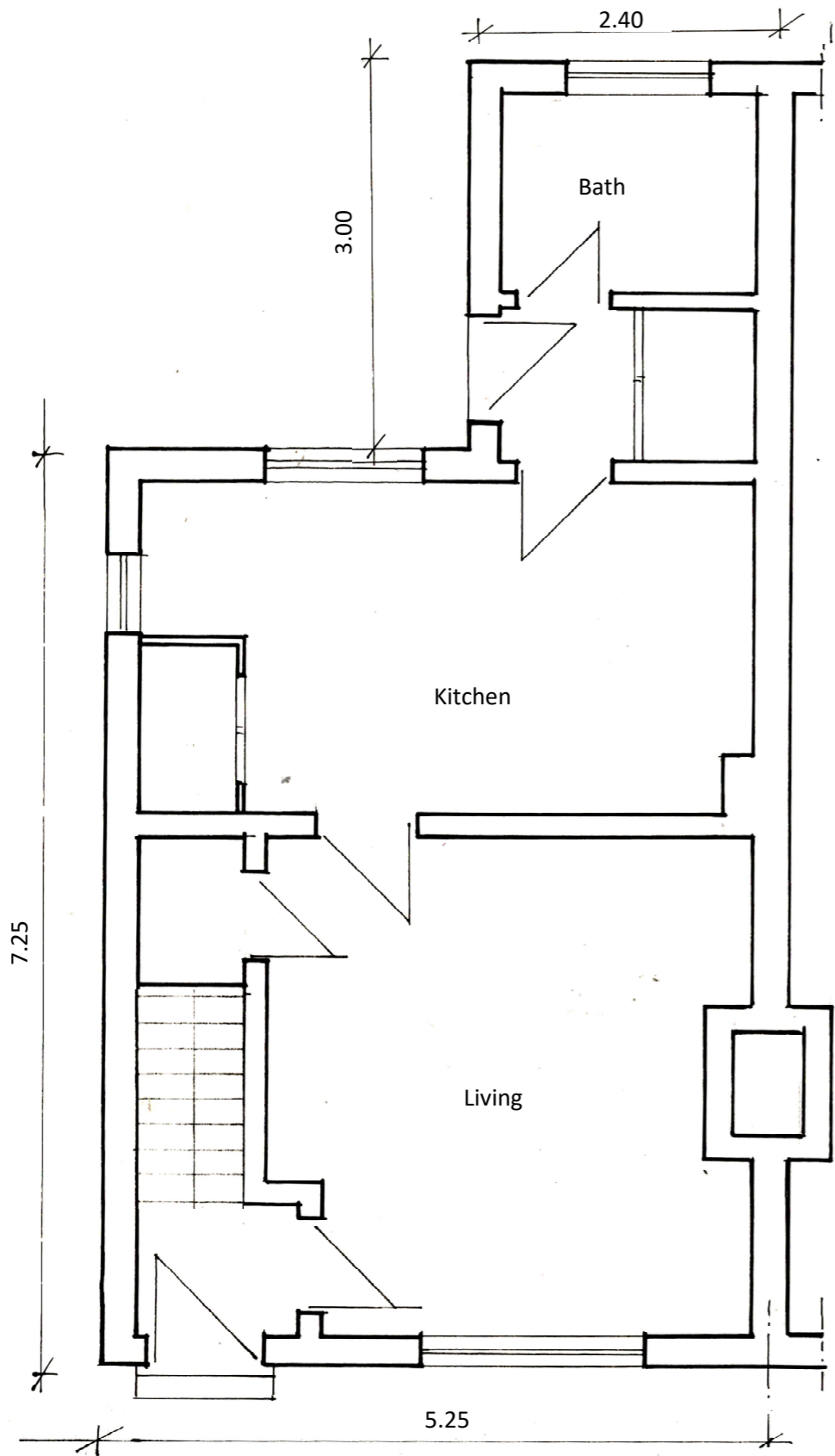
GROUND FLOOR
