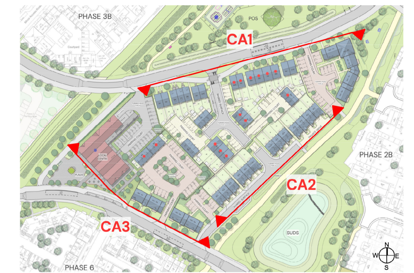
KEY PLAN
