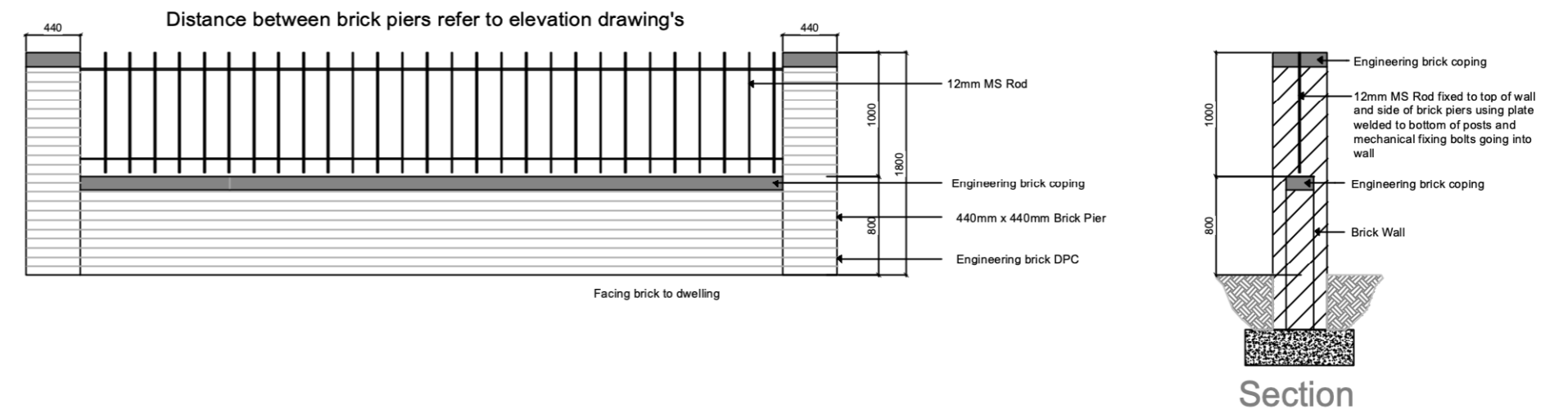
Screen 800 mm wall with 1000mm vertical bar railings - Type G
