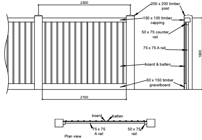
Enhanced Heavy Duty Close board Fence
