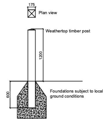
Feature timber posts
