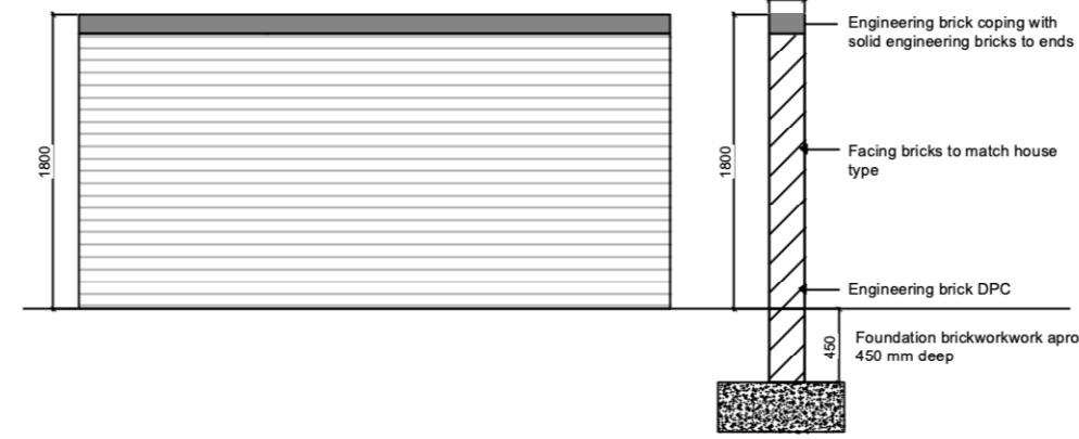
Screen Garden wall - Type A
