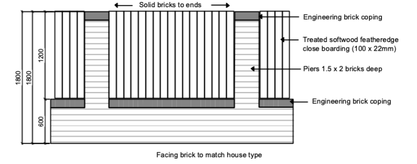
Screen Wall - Type E
