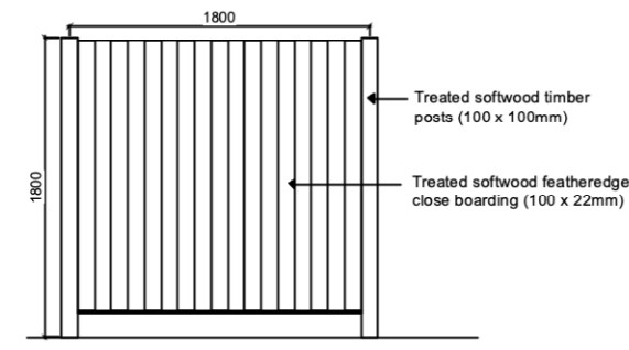
Close-boarded fence (with gravel board)
