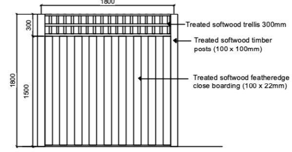
Closeboarded fence+ trellis
