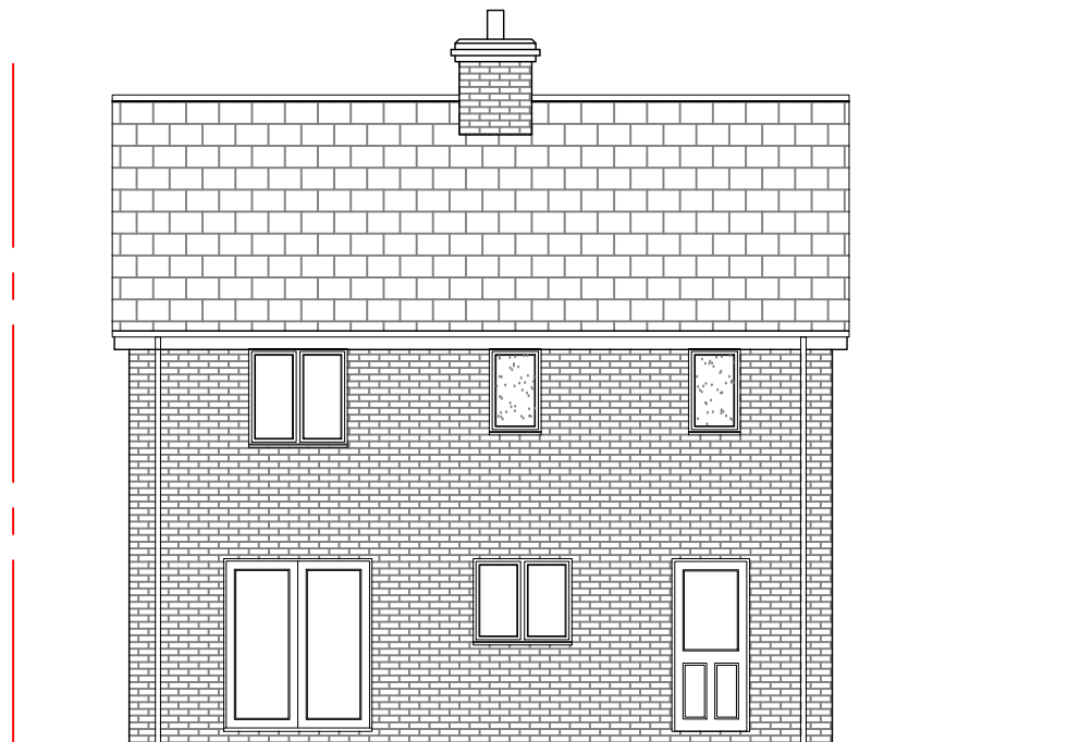
Existing Northeast Elevation
