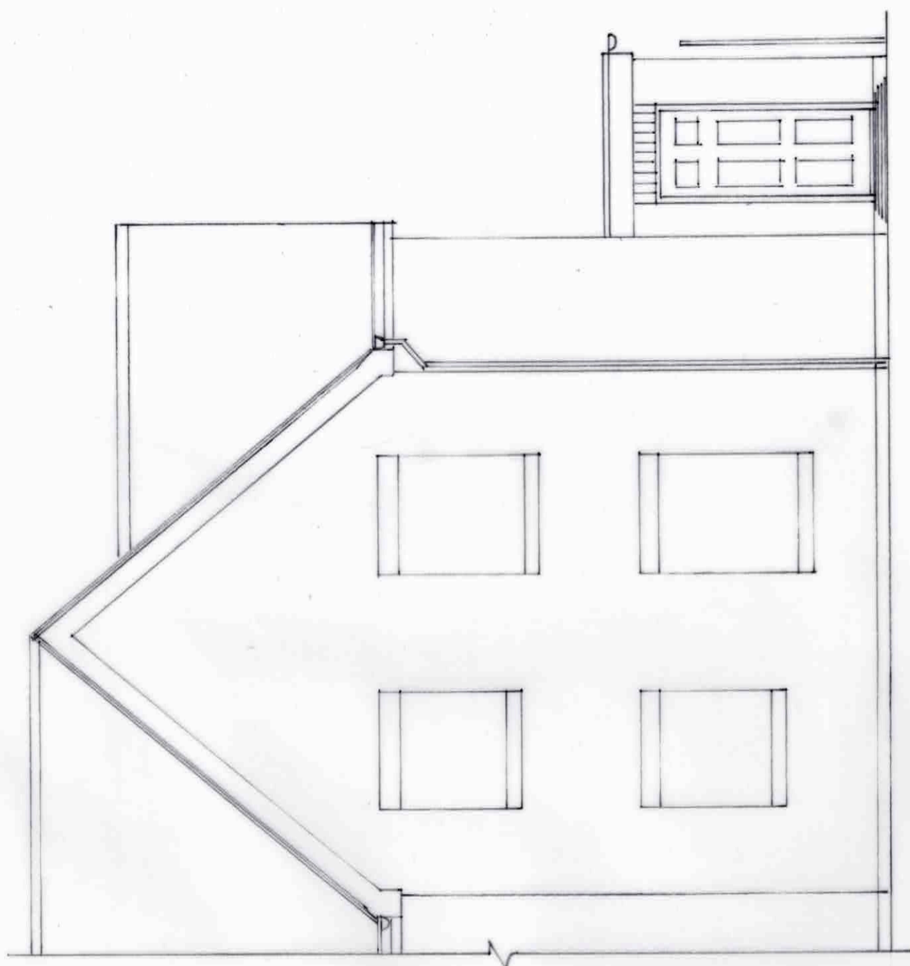
FRONT ELEVATION AS PROPOSED EXISTING
