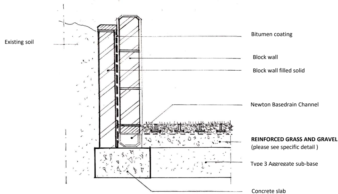
RETAINING PARKING WALL DETAIL
