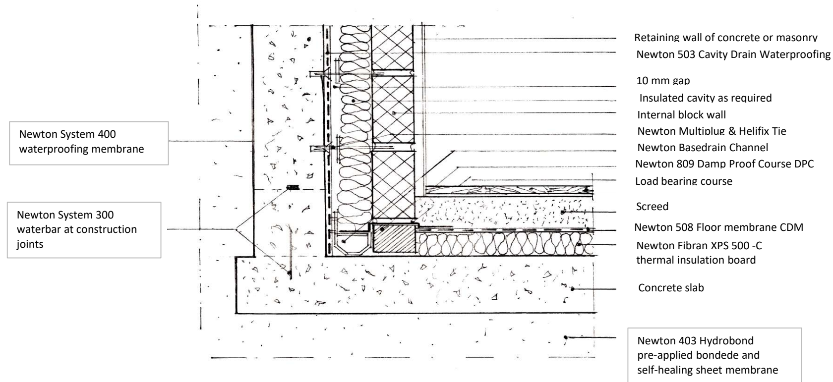
RETAINING HOUSE WALL DETAIL
