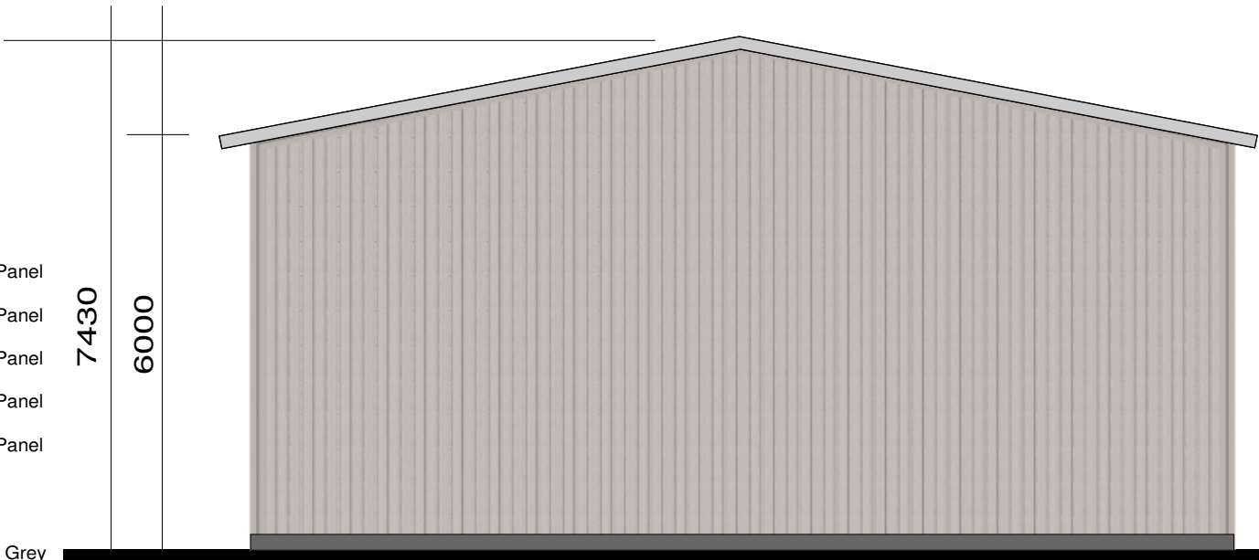
Rear Elevation
