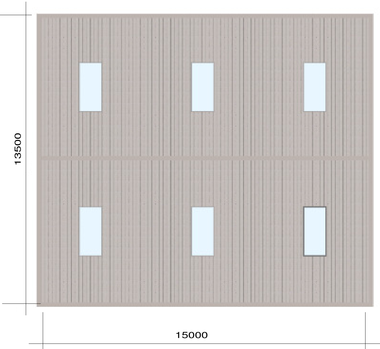
Roof Plan
