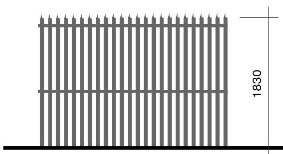
TYPICAL FENCING ELEVATION
