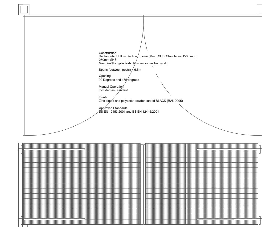
Manual double swing access gates FENCE AND BARRIER DETAILS 1:50 SCALE
