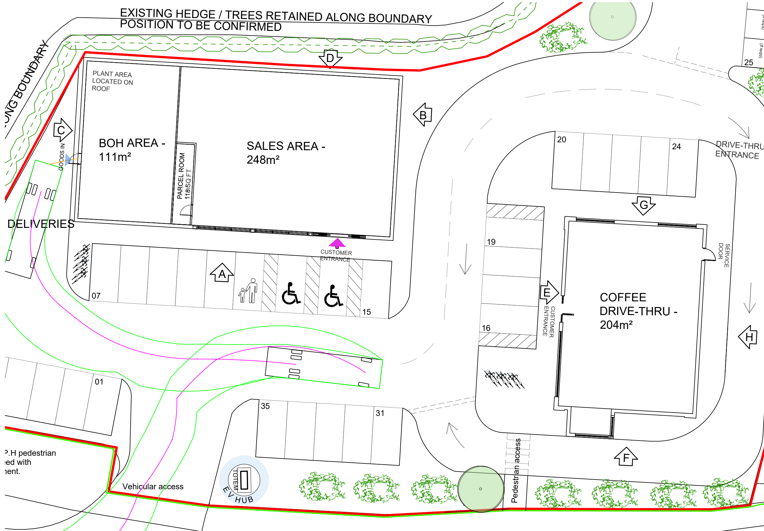
FLOOR PLAN SCALE 1:200
