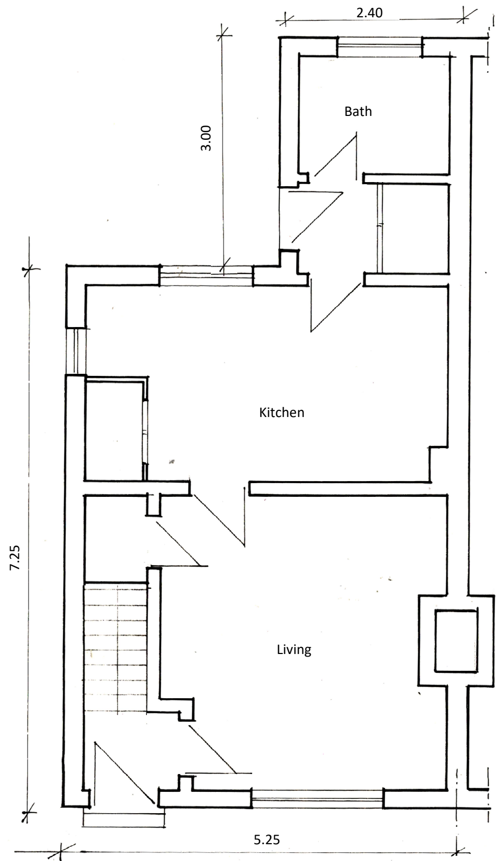
GROUND FLOOR
