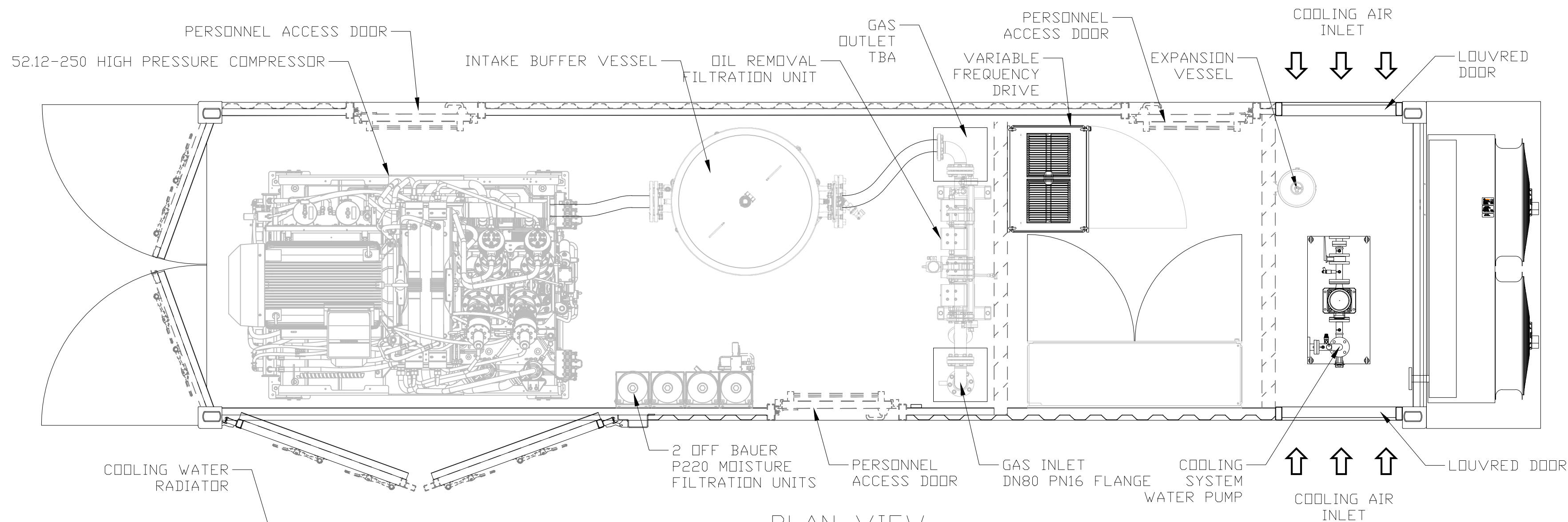
PLAN VIEW ROOF DUCTING OMITTED FOR CLARITY
