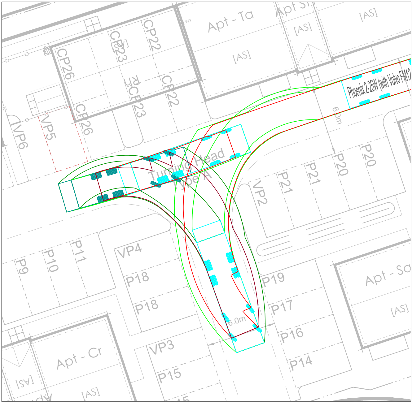
Refuse Tracking Location 1 Scale: 1:200
