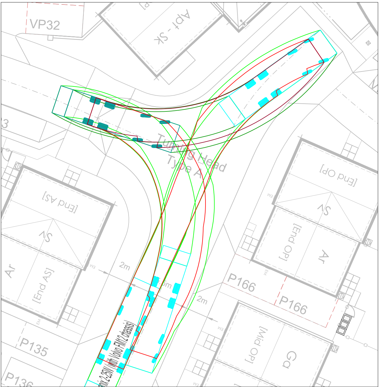
Refuse Tracking Location 4 Scale: 1:200
