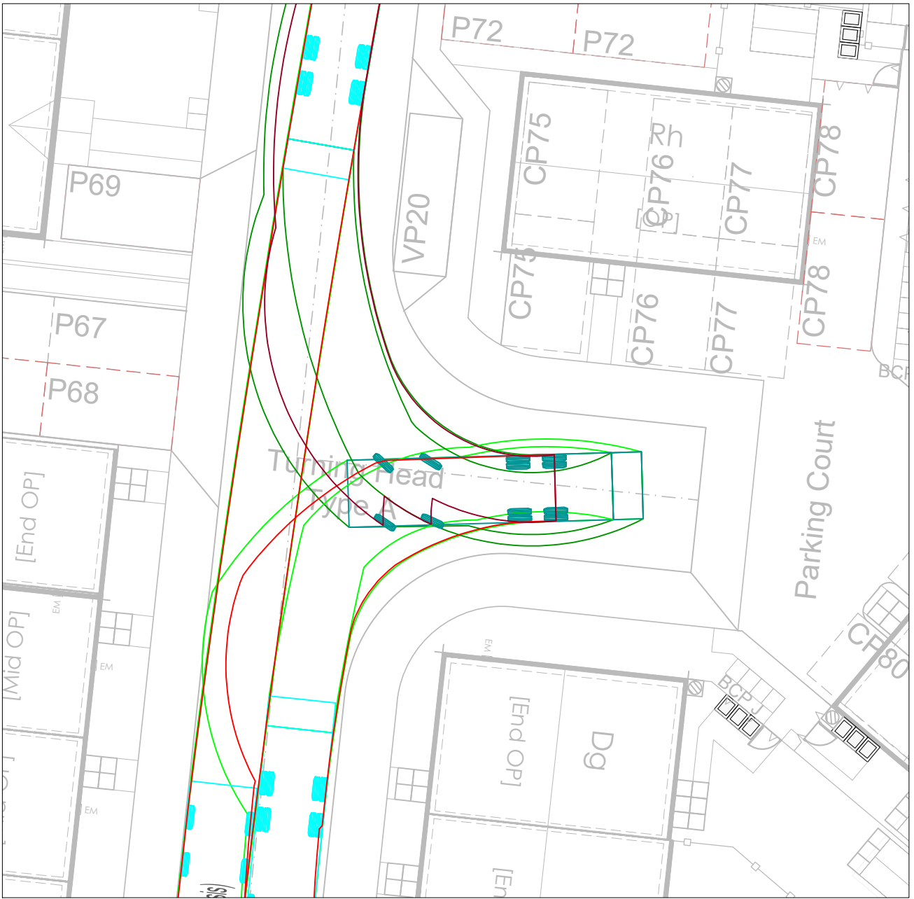
Refuse Tracking Location 2 Scale: 1:200
