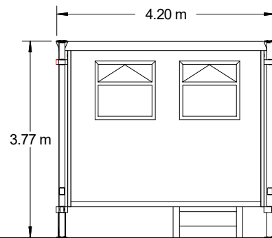
West Elevation
