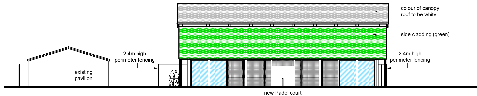
south east facing elevation as proposed - 1:200
