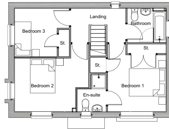
First Floor Plan (H)
